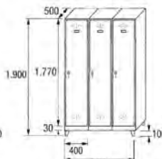
SV-40/3 COD. 44003
