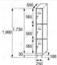
SM-25/1 COD. 42531
