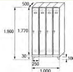
SV-25/4 COD. 42504
