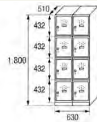
LC-30/2 COD. 73022
