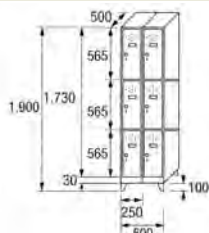
SM-25/2 COD. 42532
