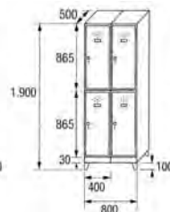
ST-40/2 COD. 44012
