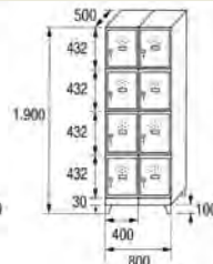
SC-40/2 COD. 44022
