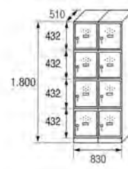
LC-40/2 COD. 74022
