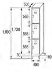
SM-40/1 COD. 44031
