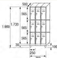
SM-25/3 COD. 42533
