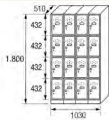
LC-25/4 COD. 72524
