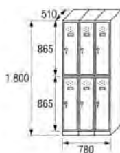
LT-25/3 COD. 72513
